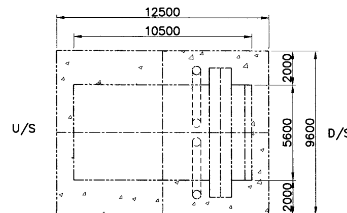
TYPICAL SECTION A-A (SCALE= 1:225)
